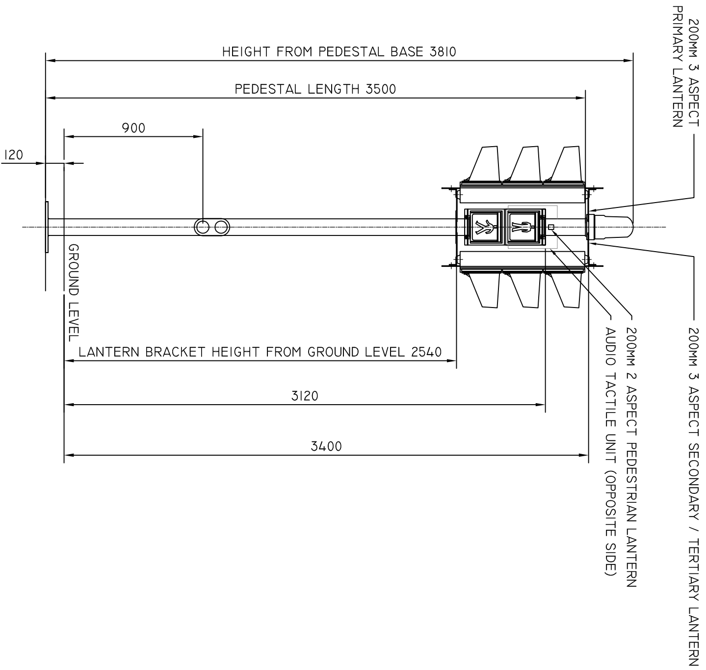
2T PEDESTAL FRONT SIDE SHOWING PEDESTRIAN LANTERN
